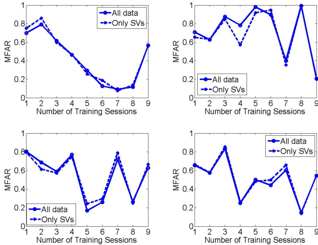
Fig. 3. The SVM test performance in terms of minimum false alarm rate at zero miss (MFAR) as a function of the number of training sessions for four subjects. The solid curve is the batch learning (uses all previous data for training) performance and the dash curve is the incremental learning (only the SVs are propagated) performance. The naive learning performance is the first dot for one training session.
