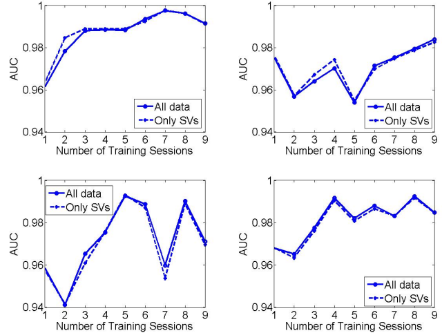
Fig. 2. The SVM test performance in terms of area under ROC (AUC) as a function of the number of training sessions for four subjects. The solid curve is the batch learning (uses all previous data for training) performance and the dash curve is the incremental learning (only the SVs are propagated) performance. The naive learning performance is the first dot for one training session.
