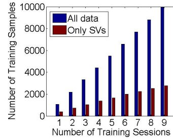
Fig. 4. The number of training samples for different number of training sessions for subject 1 using the batch learning (uses all previous data for training) and the incremental learning (only the SVs are propagated)
